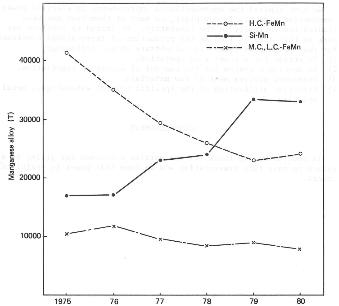
Fig. 1. Production of manganese alloys at Kobe Steel
