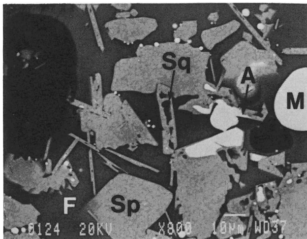
Fig. 7. SEM micrograph of the outer region of an R1A pellet tested at a \text{CO}/\text{CO}_2 ratio of 3 for 1\frac{1}{2} hours at 1300^\circ\text{C} . The formation of the sesquioxide by the direct oxidation of the ferrochromium blebs can be seen at point A
