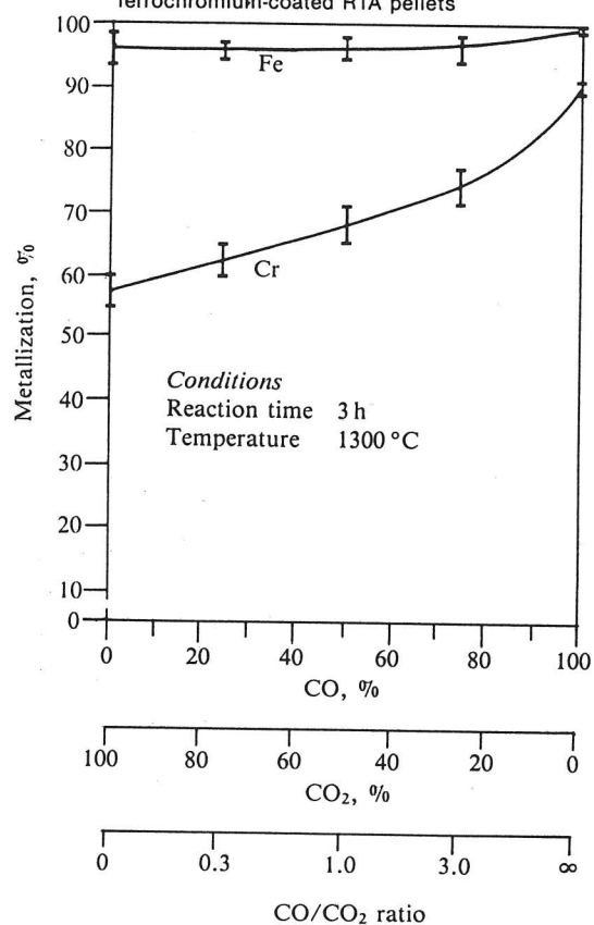
Fig. 3. Effect of the CO/CO 2 ratio on the degree of metallization of chromium and iron in reduced, ferrochromium-coated R1A pellets
