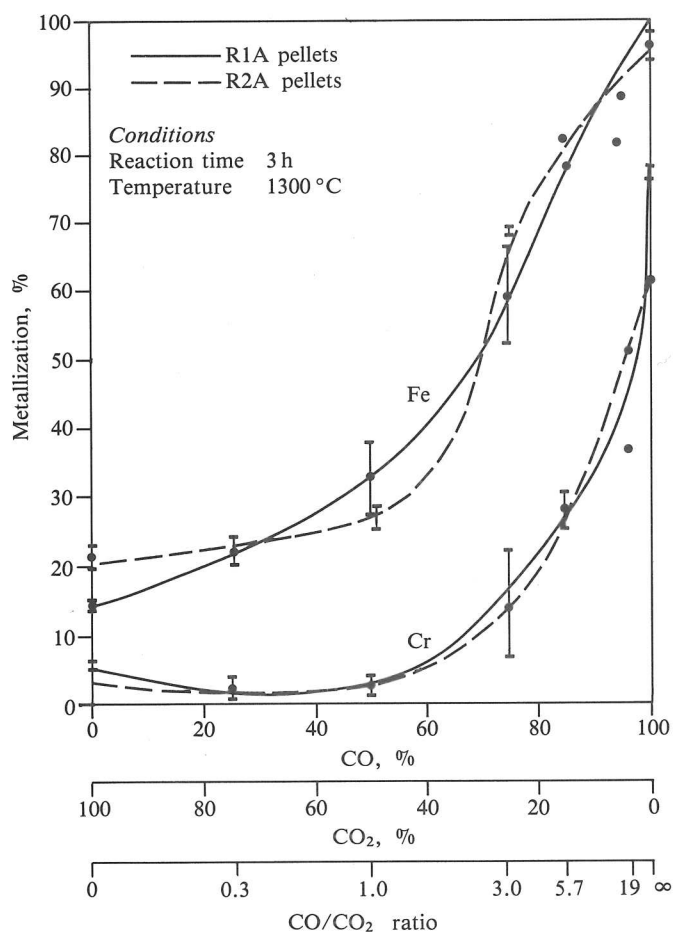
Fig. 1. Effect of the CO/CO 2 ratio on the degree of metallization of chromium and iron in reduced, uncoated R1A and R2A pellets
