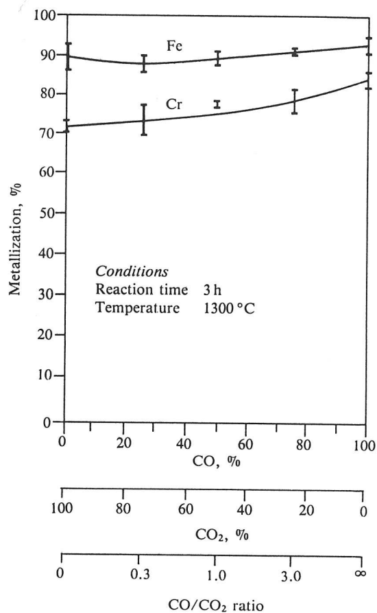
Fig. 3. Effect of the CO/CO 2 ratio on the degree of metallization of chromium and iron in reduced, ferrochromium-coated R1A pellets
