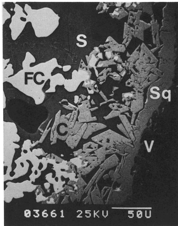
Fig. 9. SEM micrograph showing the outer layers of the ferrochromium coating in more detail.
