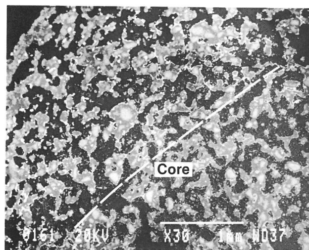
Fig. 6. SEM micrograph of an uncoated R1A pellet tested at a CO/CO 2 ratio of 3 for 1 hour at 1300 °C. The boundary between the less metallized core and the outer region of the pellet is indicated
