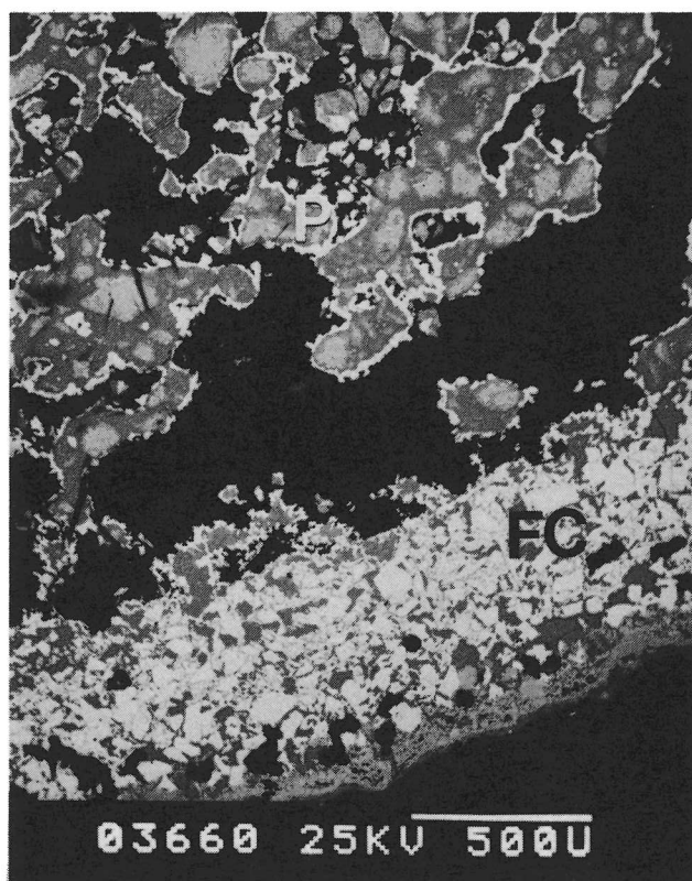
Fig. 8. SEM micrograph of a ferrochromium-coated R1A pellet tested at a \text{CO}/\text{CO}_2 ratio of 1 for 3 hours at 1300^\circ\text{C} . The boundary between the highly metallized base pellet (P) and the ferrochromium coating (FC) is clearly indicated
