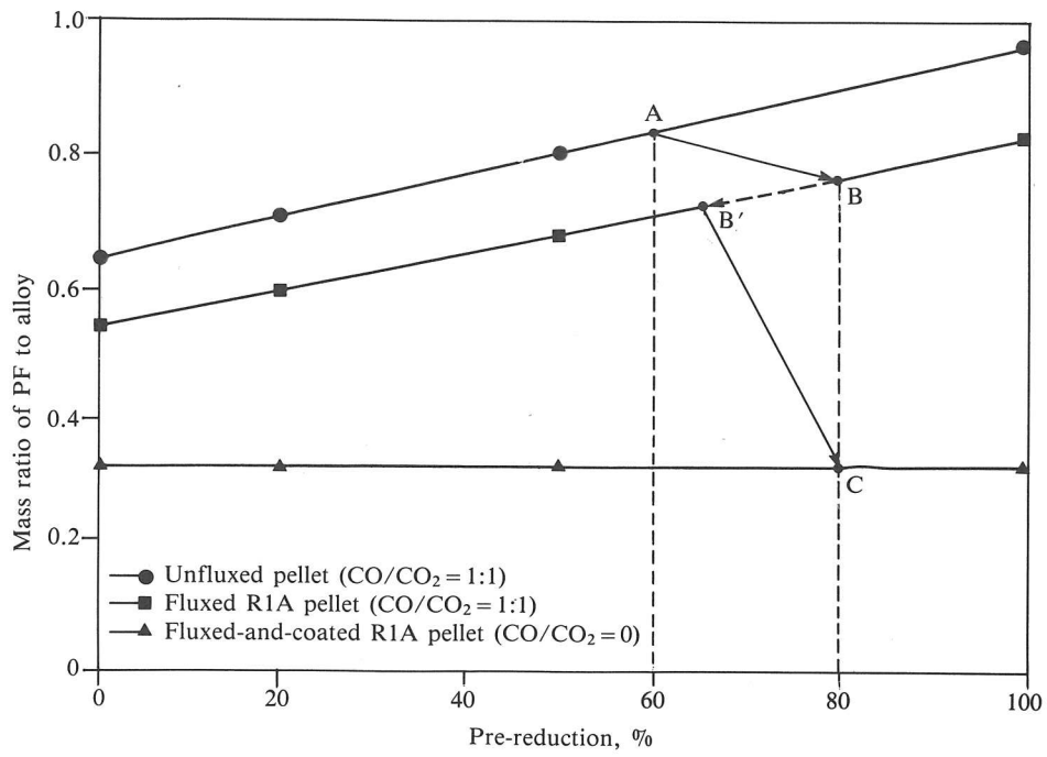
Fig. 11. Mass ratio of pulverized coal (PF) to ferrochromium required for varying levels of pre-reduction of unfluxed, fluxed, and fluxed-and-coated composite chromite pellets
