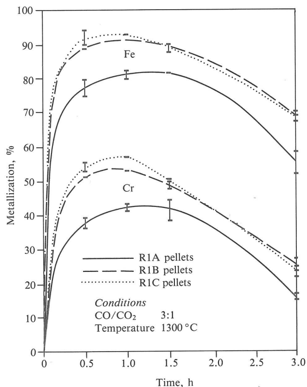
Fig. 2. Effect of reaction time on the degree of metallization of chromium and iron in reduced, uncoated R1A, R1B, and R1C pellets
