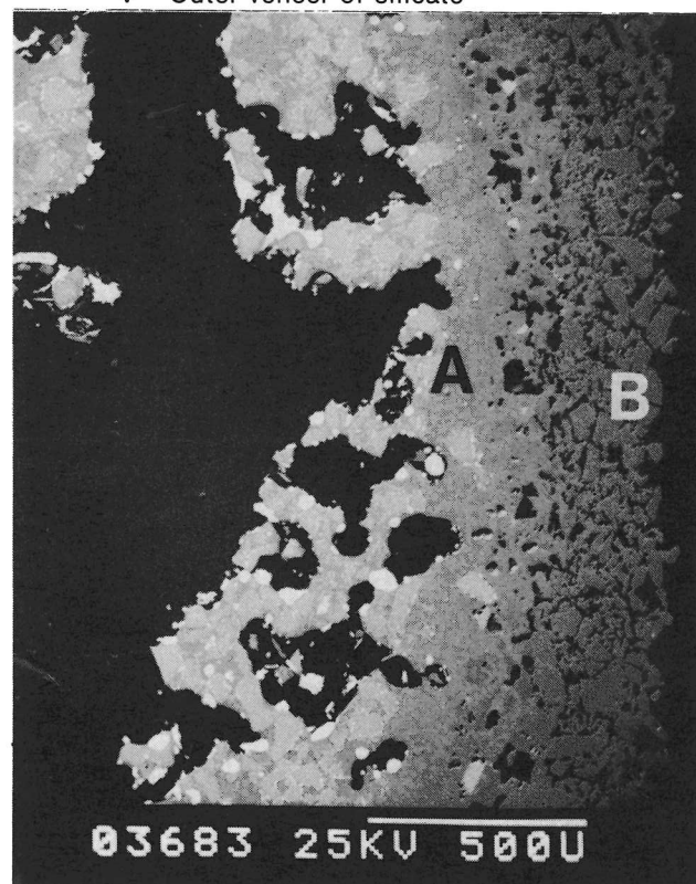
Fig. 10. SEM micrograph of an andalusite-coated R1A pellet tested under a 100 per cent \text{CO}_2 atmosphere ( \text{CO}/\text{CO}_2 = 0 ) for 3 hours at 1300^\circ\text{C} . The dense inner zone (A) and the open-textured outer zone (B) are indicated
