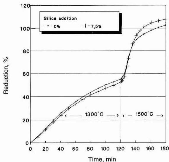
FIGURE 6. Effect of silica addition on a stagewise reduction
