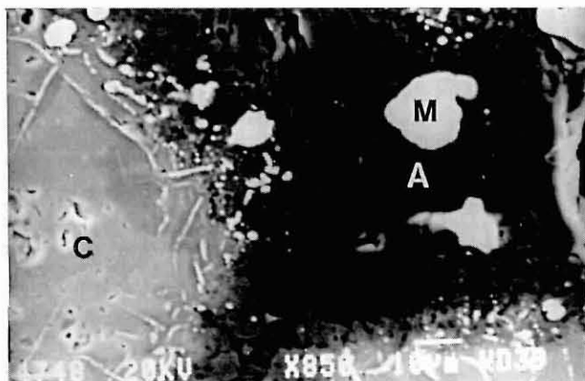
FIGURE 13. Secondary electron image of chromite particles reduced with char to 35 per cent C = Chromite M = Metal A = Slag
