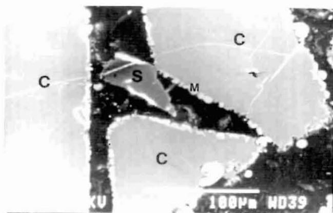
FIGURE 2. Secondary electron image of chromite particles reduced to 45 per cent at 1300°C in the presence of silica particles C = Chromite S = Silica M = Metal
