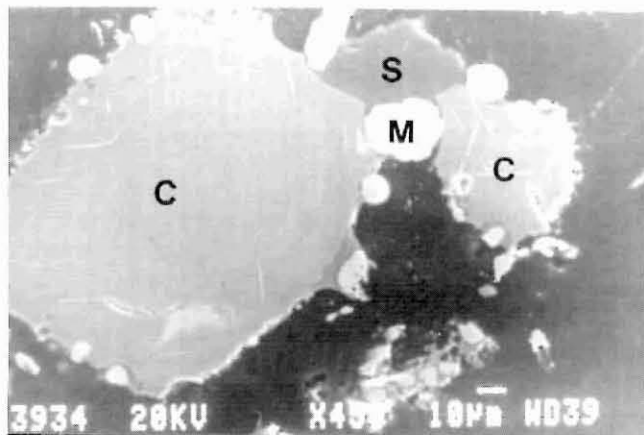
FIGURE 7. Secondary electron image of chromite particles reduced to 20 per cent at 1500°C in the presence of silica particles
