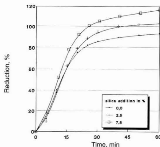
FIGURE 3. Effect of silica addition on reduction curves at 1500°C
