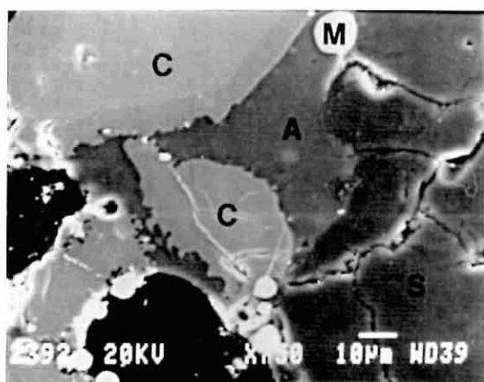
FIGURE 9. Secondary electron image of a silica-slag phase forming at the interface of a chromite particle reduced to 20 per cent C = Chromite S = Silica M = Metal A = Slag
