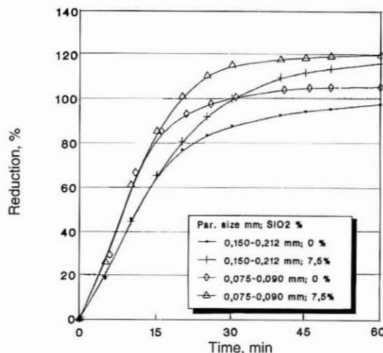
FIGURE 4. Effect of silica addition on the reduction of chromite at 1500°C in the particle-size range 0,150 to 0,212 mm and 0,075 to 0,090 mm
