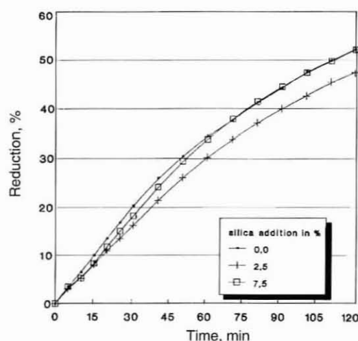
FIGURE 1. Effect of silica addition on reduction curves at 1300°C
