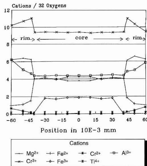
FIGURE 8. Variations in cations per 32 oxygen atoms across a particle that has undergone 20 per cent reduction
