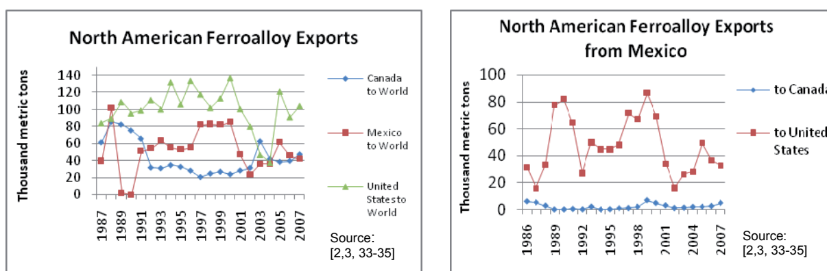
Figure 7: North American ferroalloy exports to the world.
