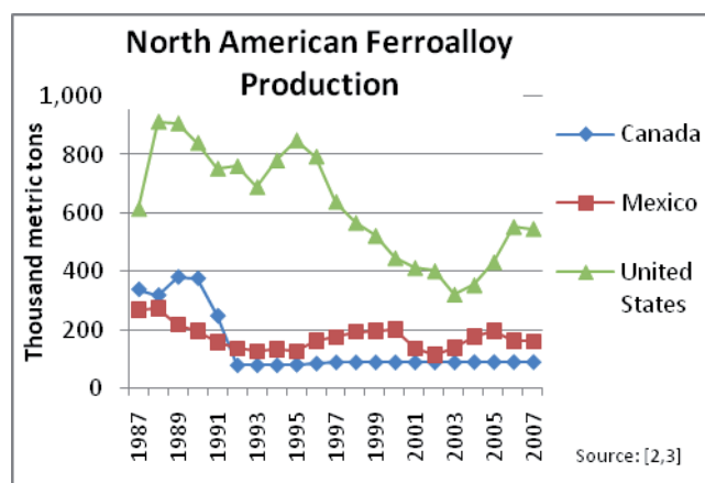
Figure 5: North American ferroalloy production.
