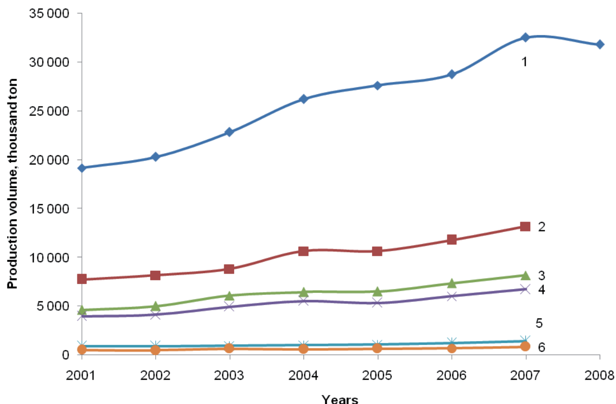
Figure 1: World ferro-alloy production volume in 2001 – 2008. 1 – total volume; 2 – manganese alloys; 3 – ferrochromium; 4 – ferrosilicon; 5 – iron nickel; 6 – silicon.
