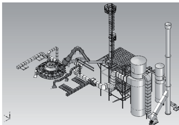
Figure 9: 3D CAD Rendering of the offgas & fume extraction area
