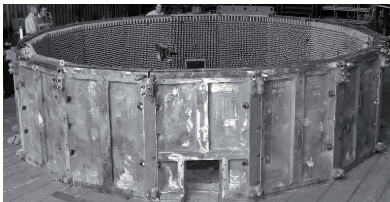
Figure 4: Shop assembly of the 12 MW DC Furnace CFM side wall cooling panels.
