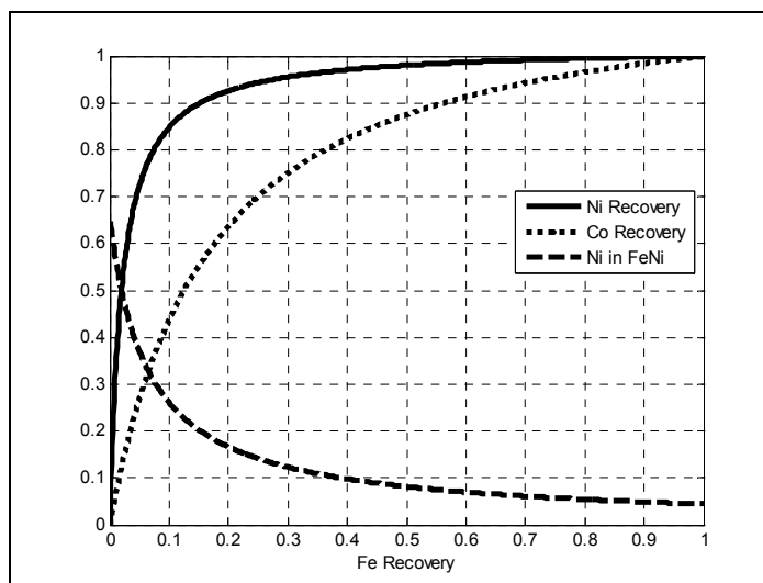
Figure 1: Relationship between Ni, Co and Fe recoveries and alloy Ni content[2][4]
