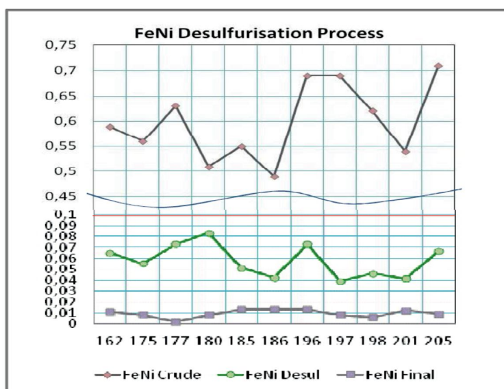
Figure 2: FeNi desulfurization process
