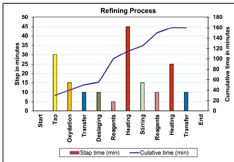
Figure 5: Summarized FeNi process
