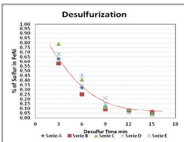
Figure 2: FeNi desulfurization process
