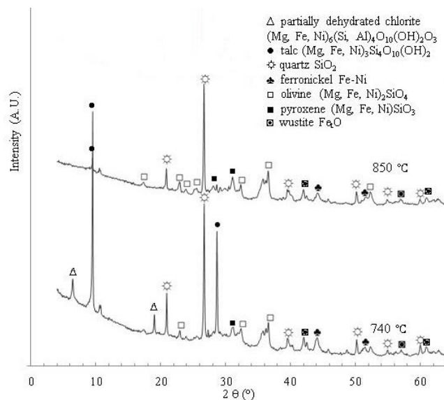
Figure 11: XRD analysis of 53-200 \mu m ore reduced at 740 and 850 °C in 60 vol% CO-40 vol% CO 2
